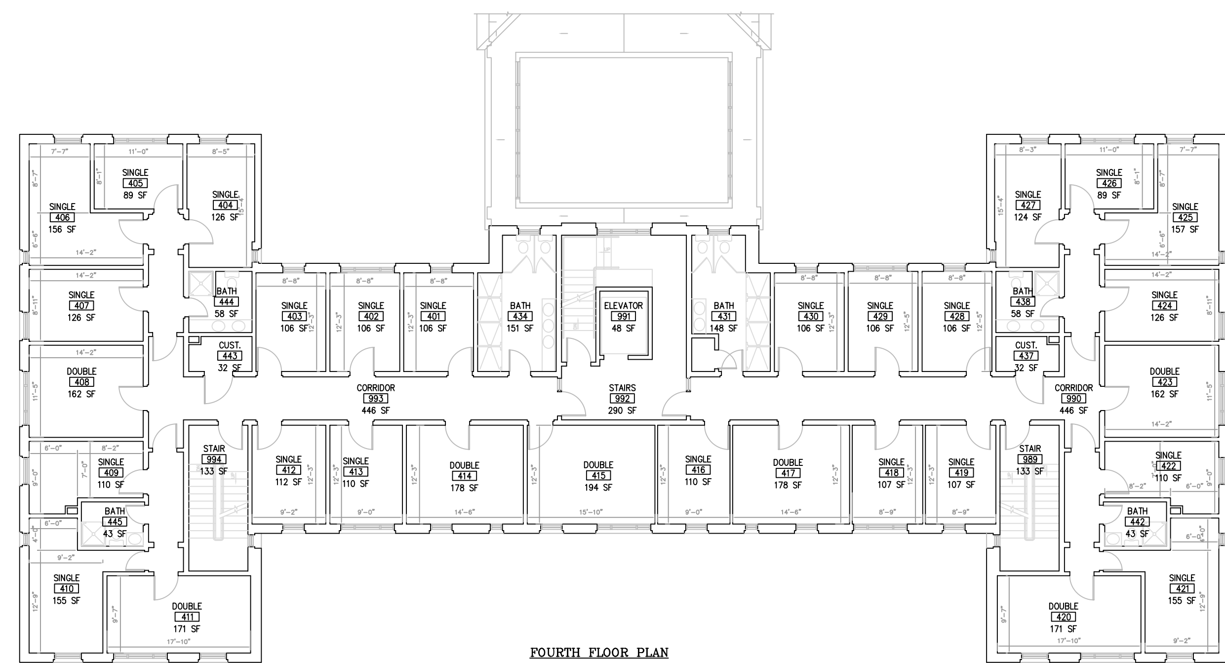
FOURTH FLOOR PLAN HEPBURN HALL
