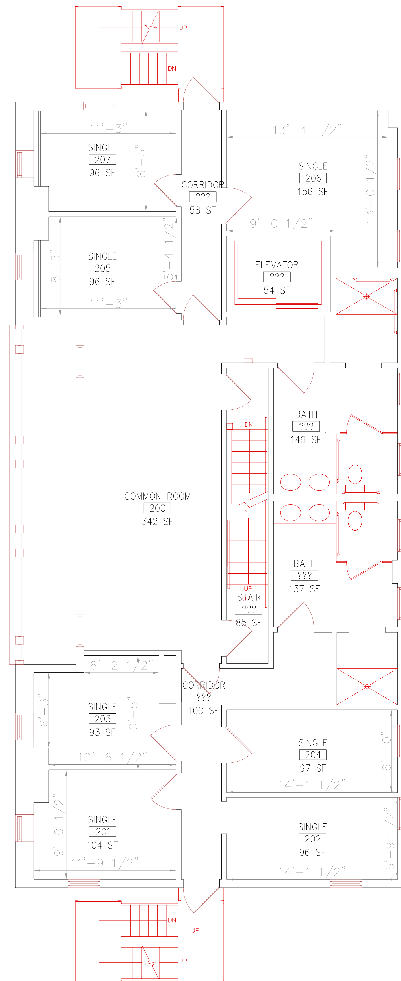
SECOND FLOOR PLAN MEEKER HOUSE
