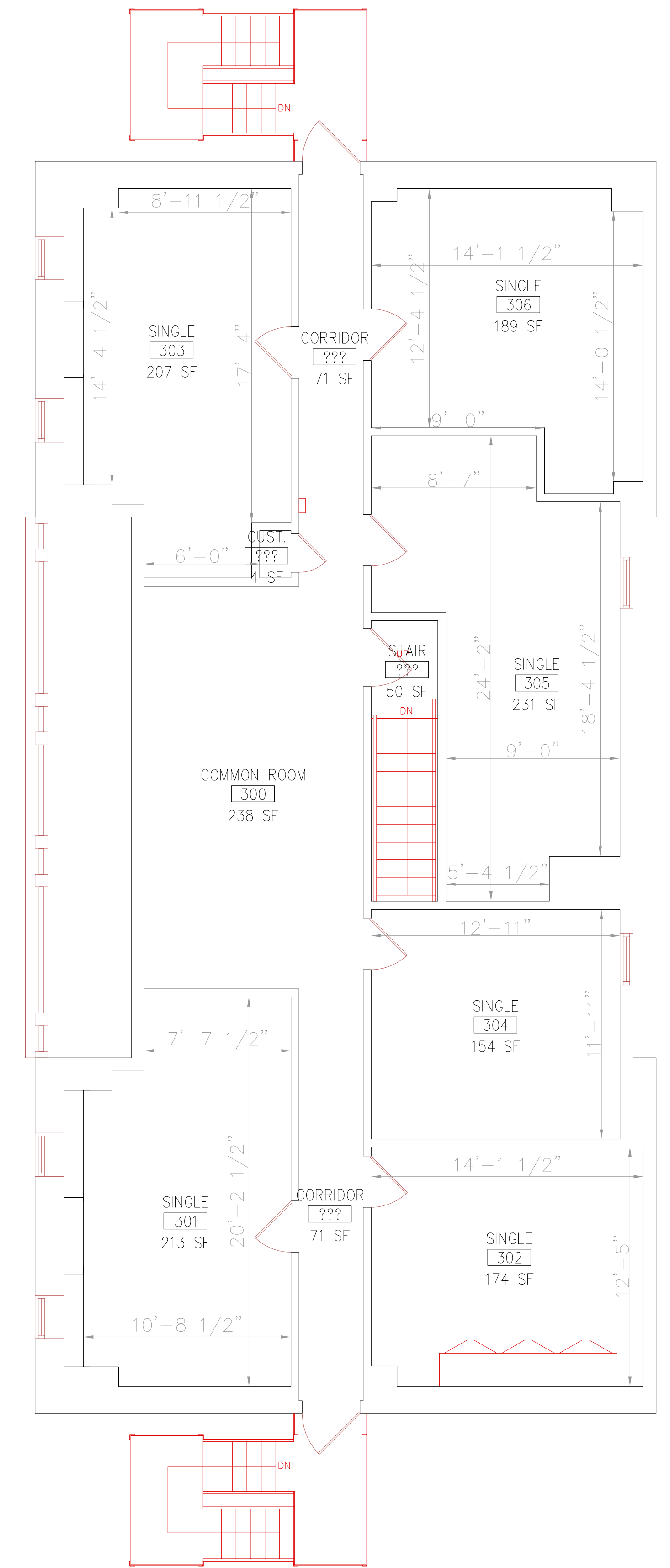
THIRD FLOOR PLAN MEEKER HOUSE
