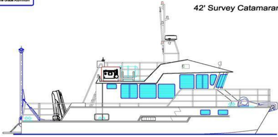
OUTBOARD PROFILE
