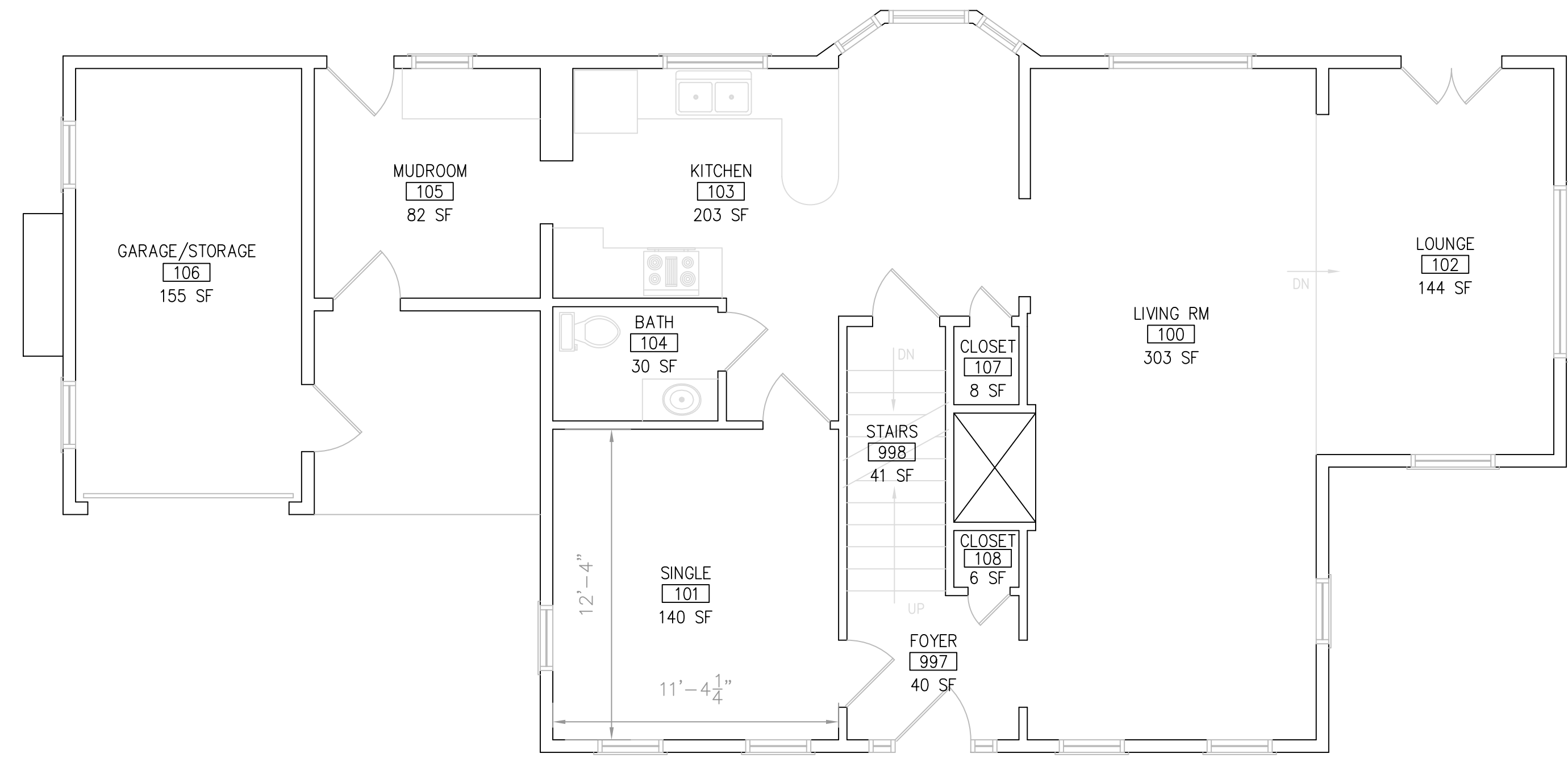
FIRST FLOOR PLAN 129 ADIRONDACK VIEW-BOWKER HOUSE
