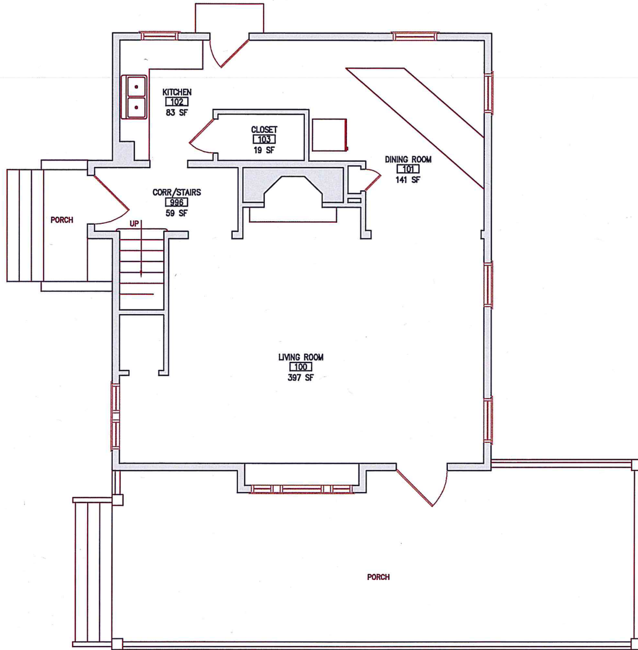
FIRST FLOOR PLAN TREMEN HOUSE
