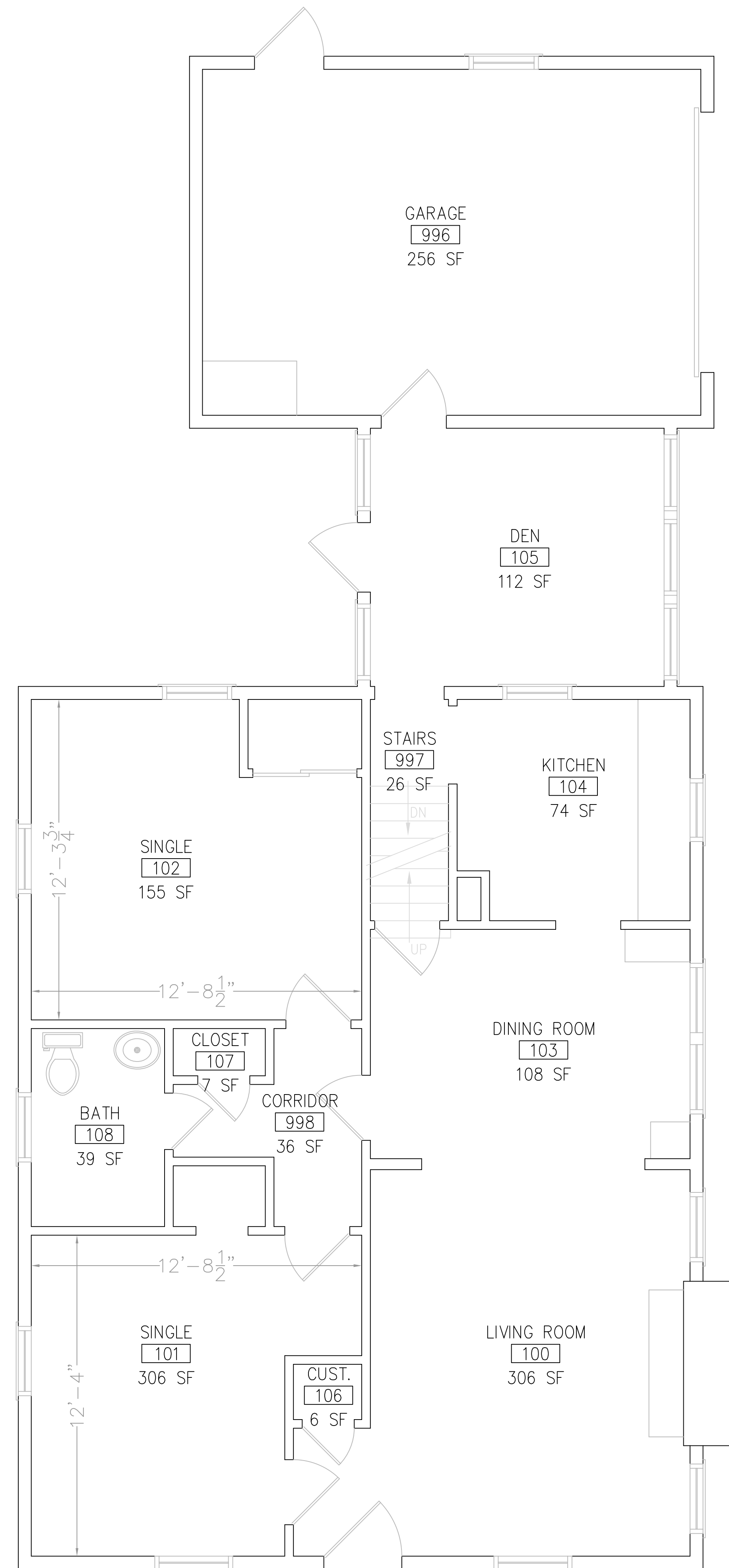
FIRST FLOOR PLAN 131 Franklin – Arabic House
