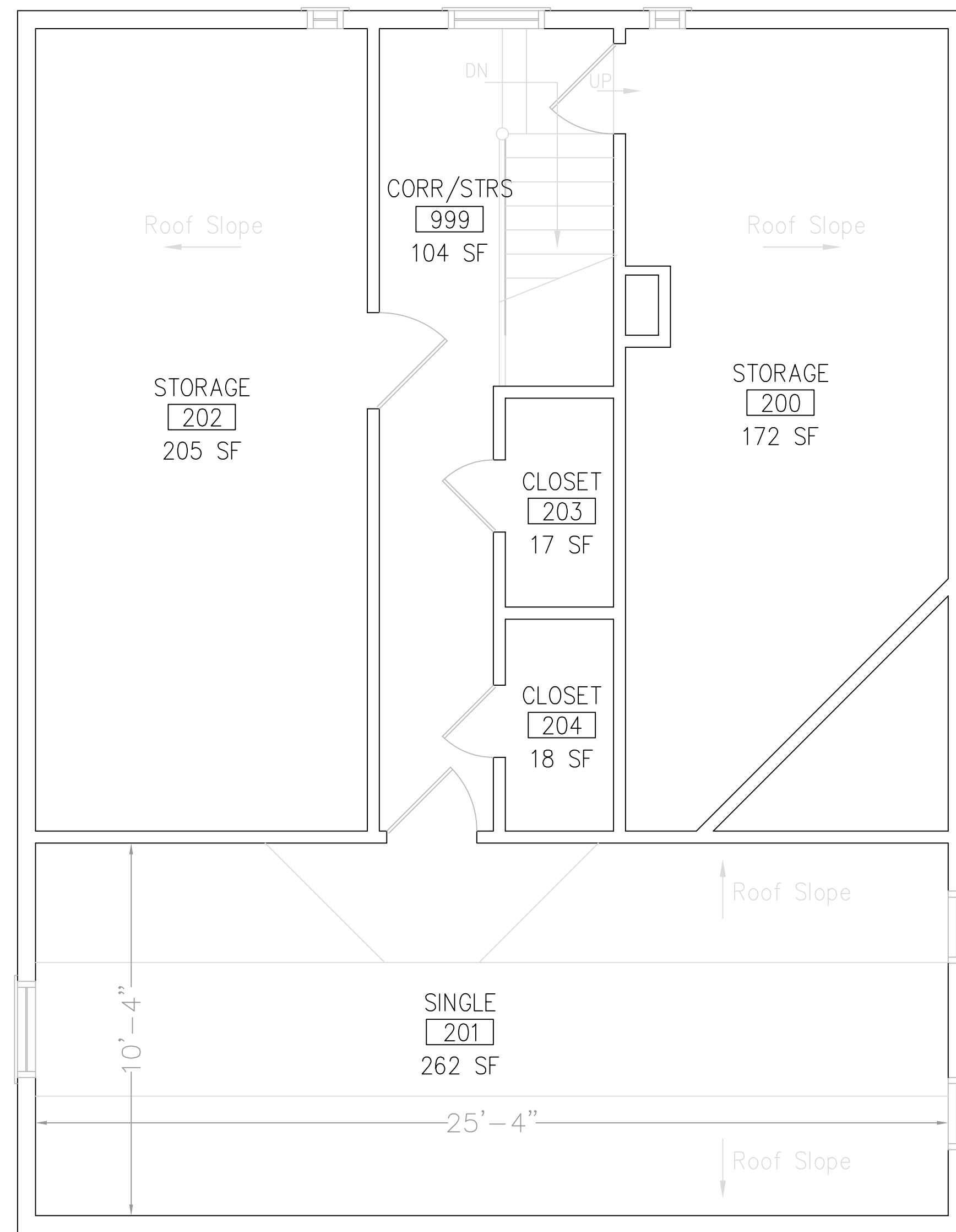
SECOND FLOOR PLAN 131 Franklin – Arabic House
